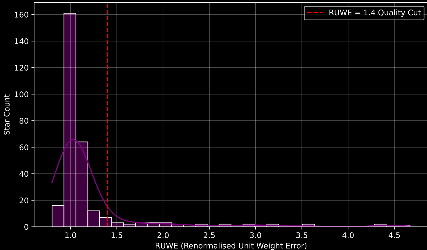
GALAH DR4 Field [76] RUWE Distribution (n= 291)
