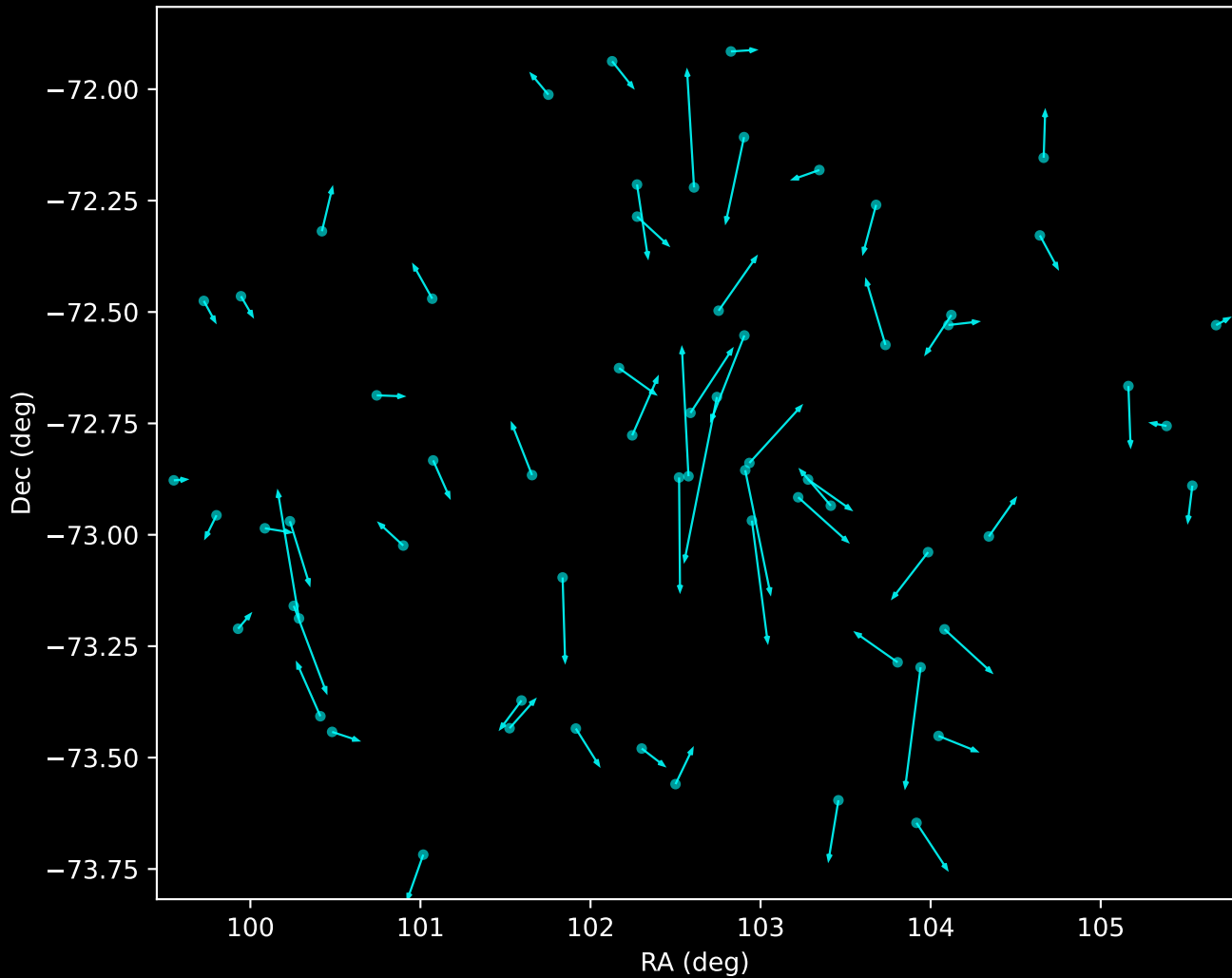
GALAH DR4 Noise Stream Proper Motion Vectors (n=64)
