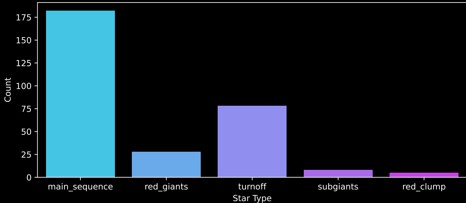
GALAH DR4 Field: [76] Count plot of Star Type
