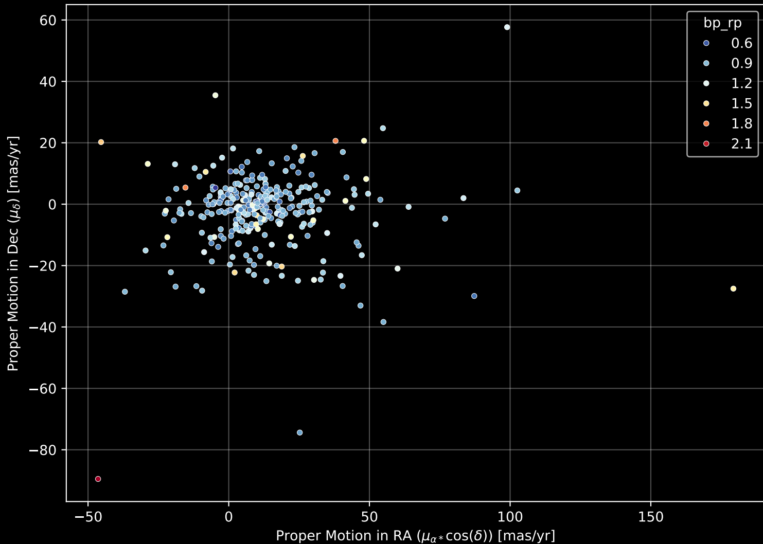
GALAH DR4 Field: [76] Proper Motion Diagram (n= 301)
