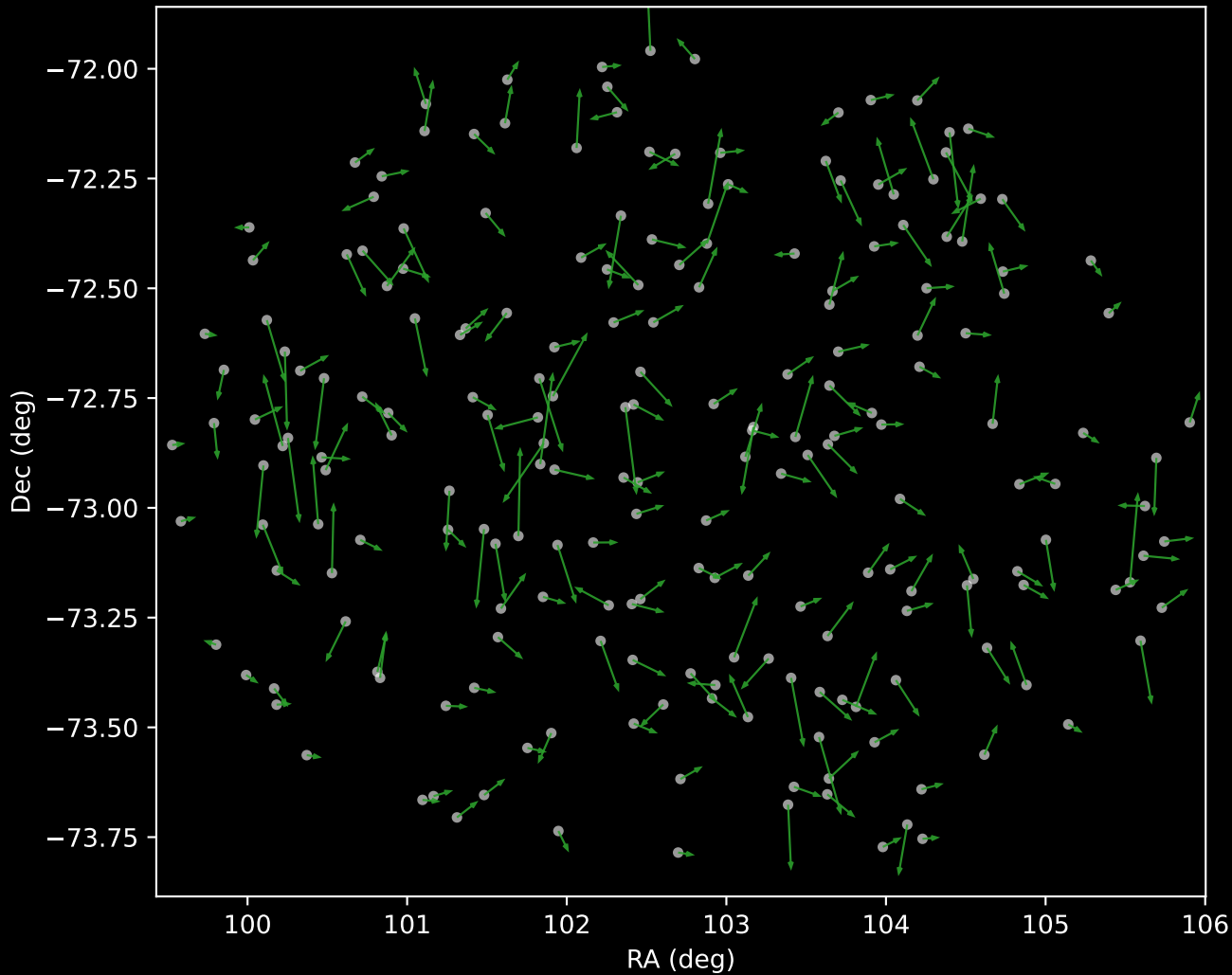
GALAH DR4 Cluster 4 Proper Motion Vectors (n=211)
