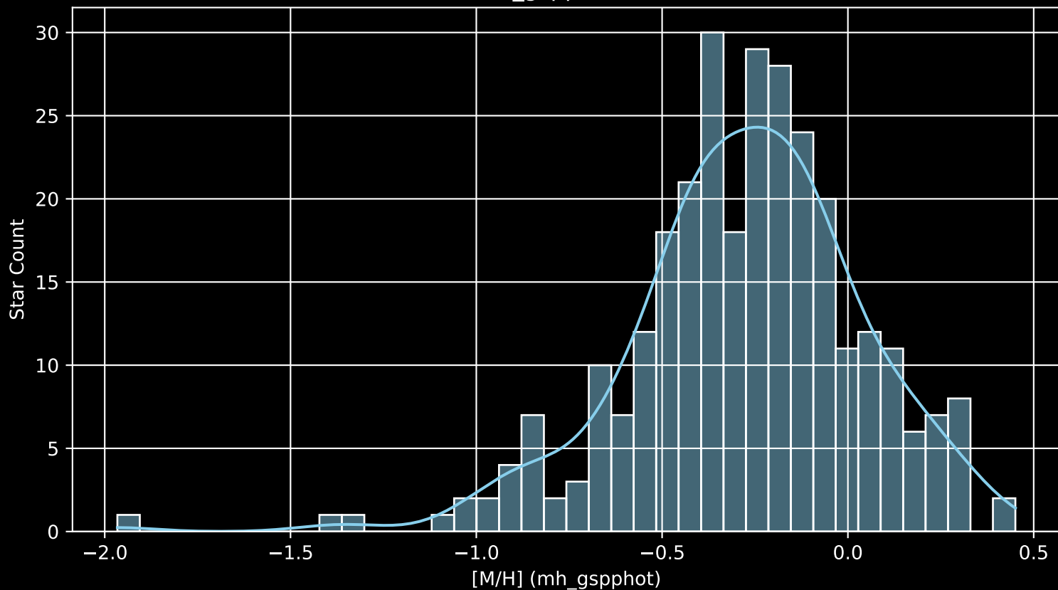
GALAH DR4 Field: [76] [M/H] (mh_gspphot) (n= 298)
